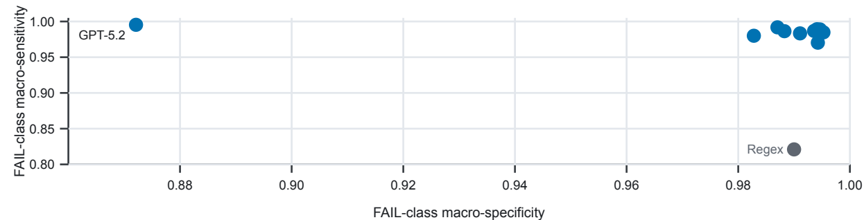
b FAIL sensitivity by model and rule
