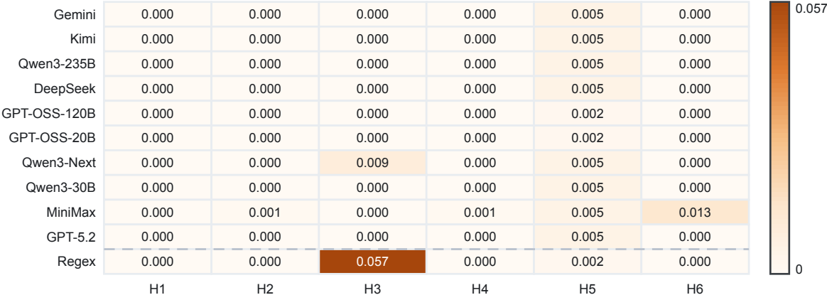
b Applicability discrimination
