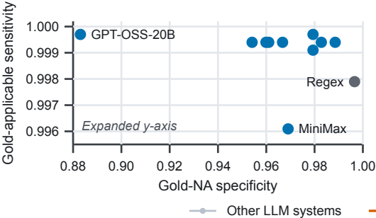
b Applicability discrimination
