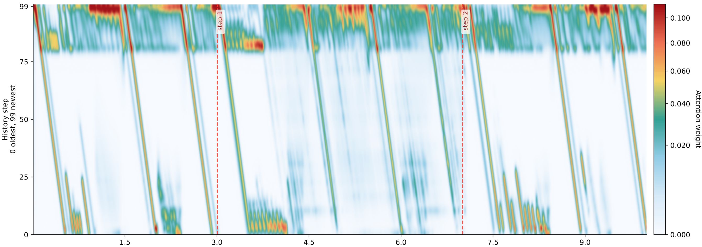
DRD-RMA Fast Branch Attention
