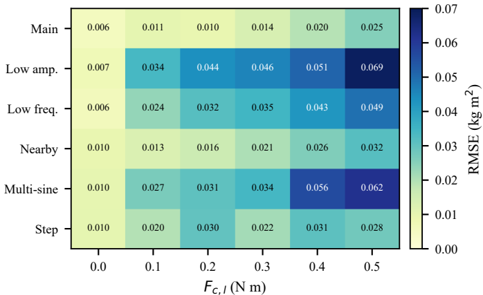
Stable-segment inertia RMSE ( \text{kg m}^2 )
