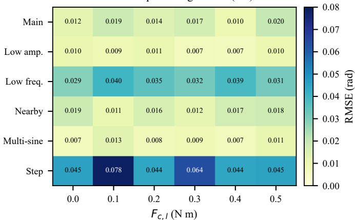
Closed-loop tracking RMSE (rad)
