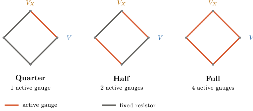
Figure 6: Quarter-, half-, and full-bridge strain-gauge arrangements. A larger number of active arms yields a larger output for a given strain and improves the cancellation of temperature and bending effects.
