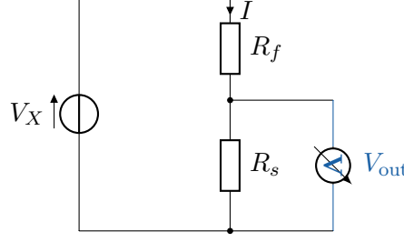
Figure 1: Ratiometric half bridge. The completion resistor R_f and the excitation V_X reside in the instrument; the sensor resistance is obtained from the ratio of V_{out} to V_X through Equation (1).
