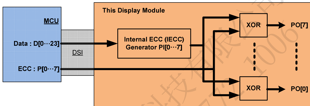
Figure 58 Internal Error Correction Code (IECC) on the Display Module (The Receiver)
