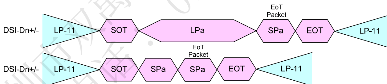
Figure 35 Single Packet in High-Speed Data Transmission with EoT packet enable
