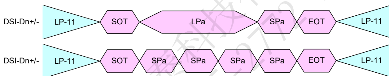
Figure 34 Multiple Packets in High-Speed Data Transmission with EoT packet disabled
