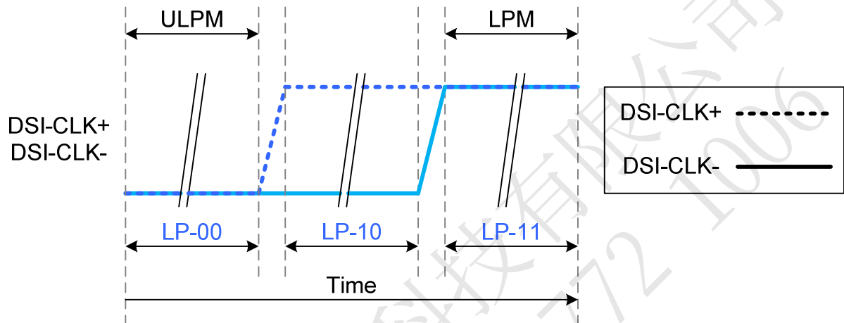
Figure 16 From ULPM to LPM
