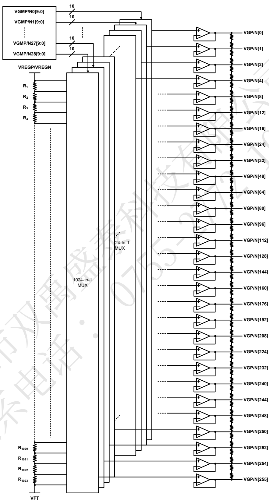
Figure 67 positive and Negative grayscale voltage generation
