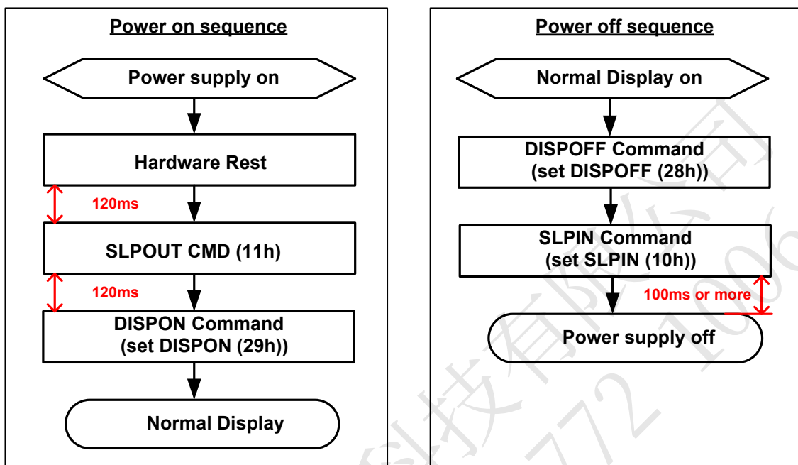
Figure 72 The power On/Off sequence block diagram
