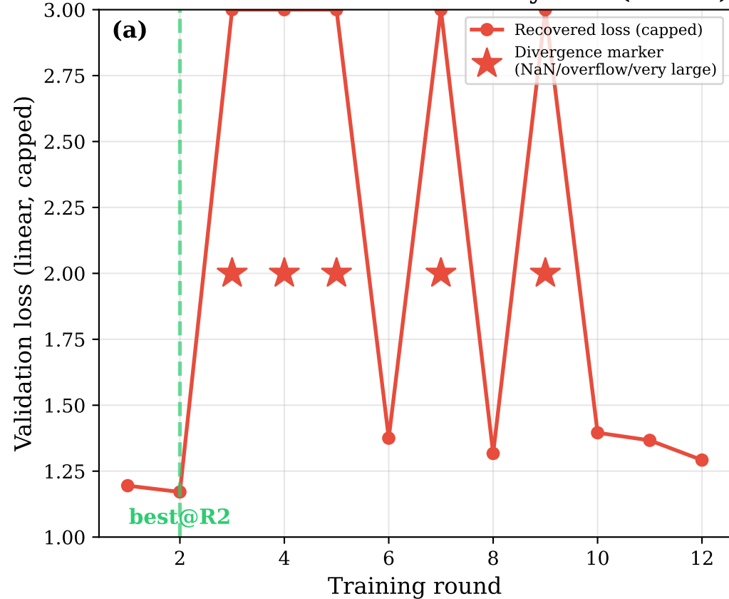
B1 Run 7: oscillation after early best (Pascal)
