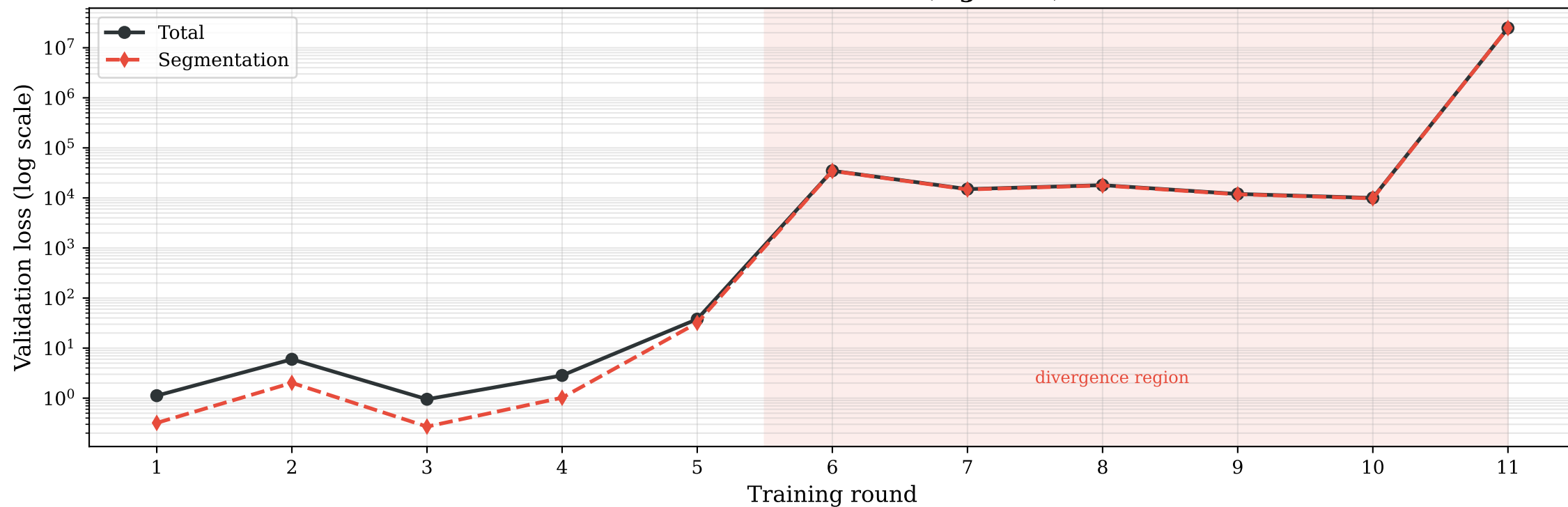
NYU: HCA full timeline (log scale)
