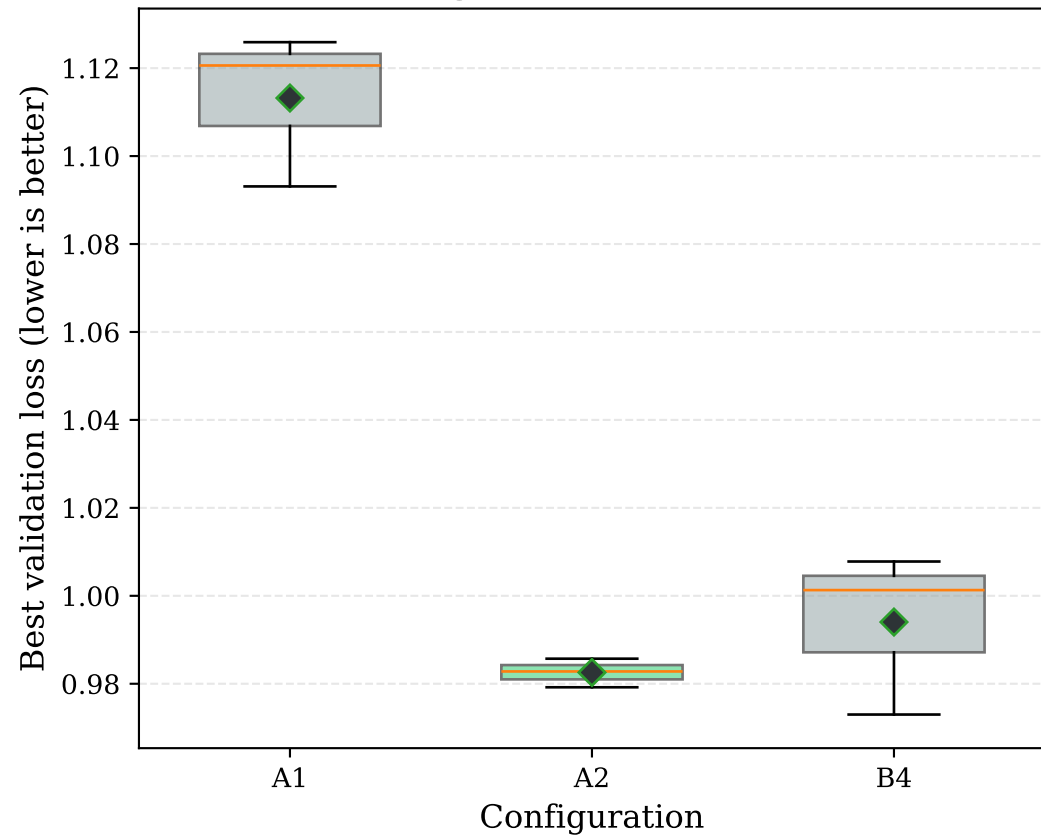
Pascal: stable configurations (three-run distribution)
