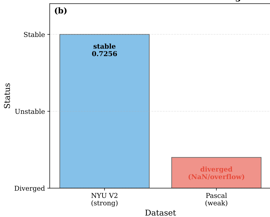
B1 across datasets: stable vs diverged
