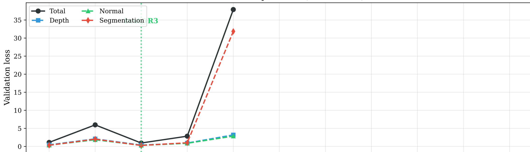
NYU: HCA early rounds (linear scale)
