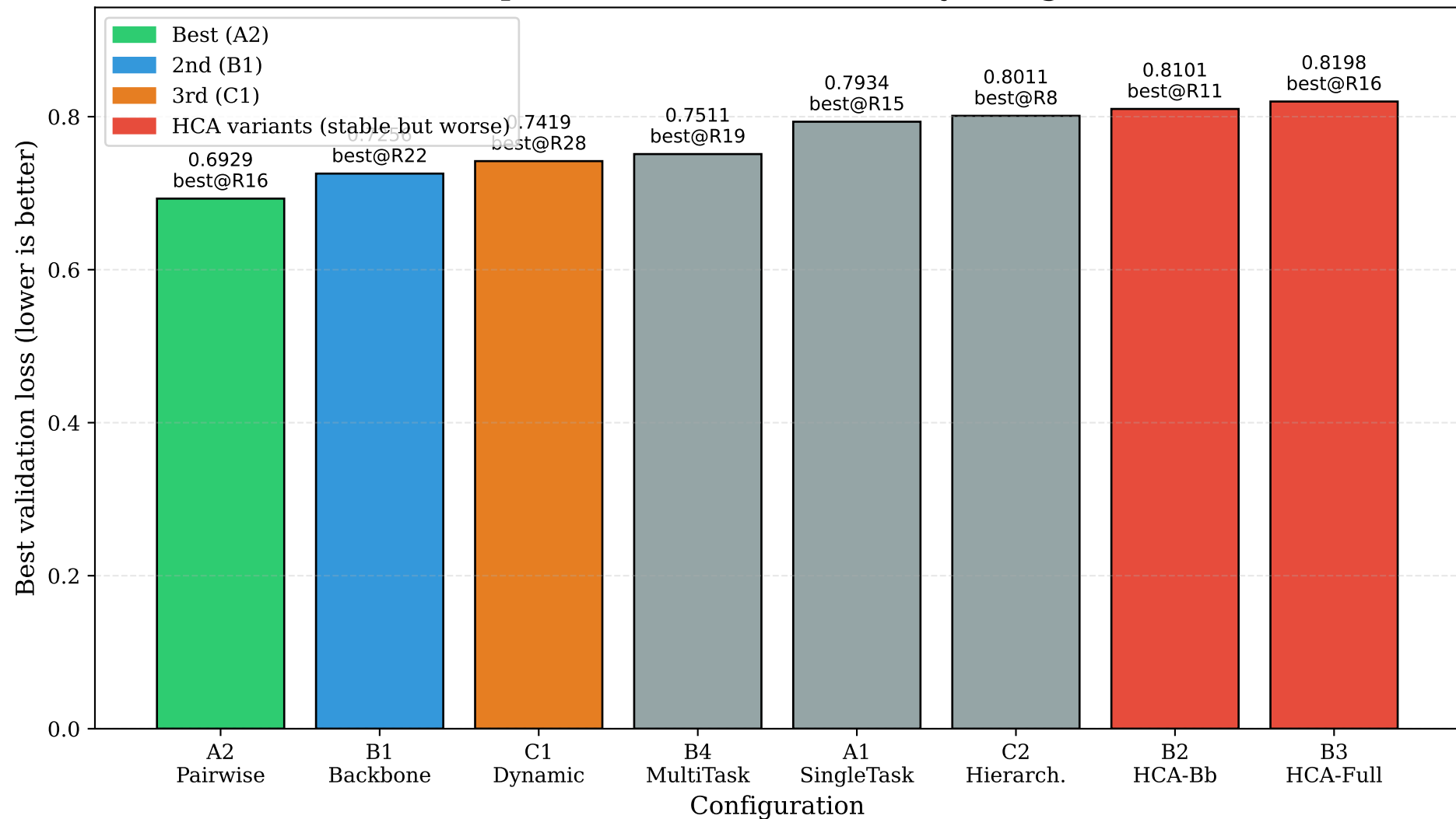
NYU Depth V2: best validation loss by configuration
