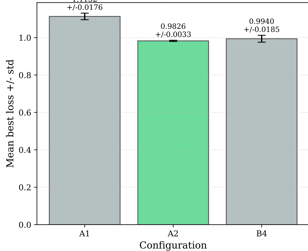
Pascal: stable configurations (mean +/- std)
