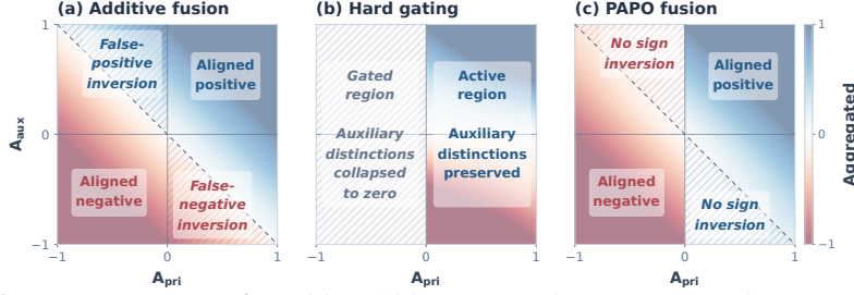
Figure 1: Advantage aggregation. (a) Additive aggregation can cause advantage priority inversion , where a dominant auxiliary signal reverses the sign induced by the primary advantage. (b) Hard gating enforces priority coarsely by discarding auxiliary distinctions for unsatisfied primary condition. (c) PAPO preserves the primary sign during fusion while retaining graded auxiliary supervision, maintaining the primary-induced preference structure.
