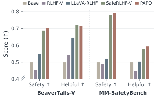
Figure 6: Multimodal safety alignment results for the Qwen2-VL-7B model.
