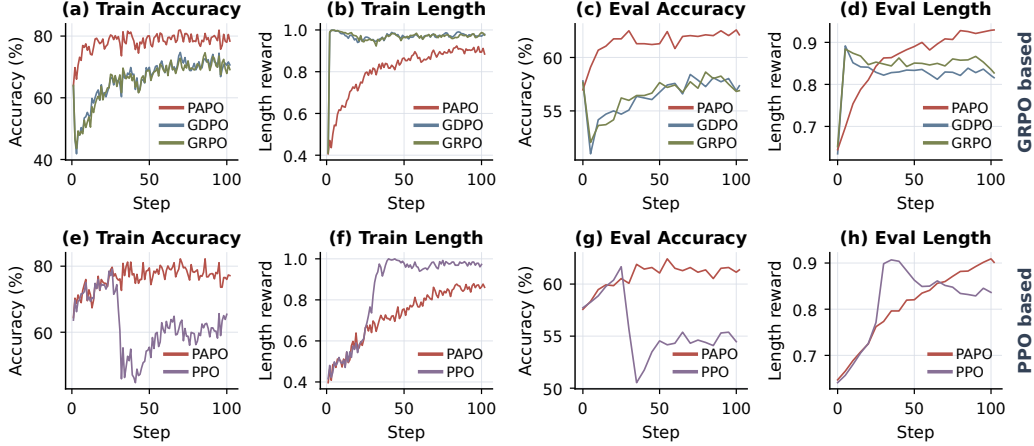
Figure 3: PAPO Dynamics. PAPO maintains the best accuracy \uparrow while having a competitive auxiliary length compliance \uparrow for GRPO-based (top) and PPO-based (bottom) methods.
