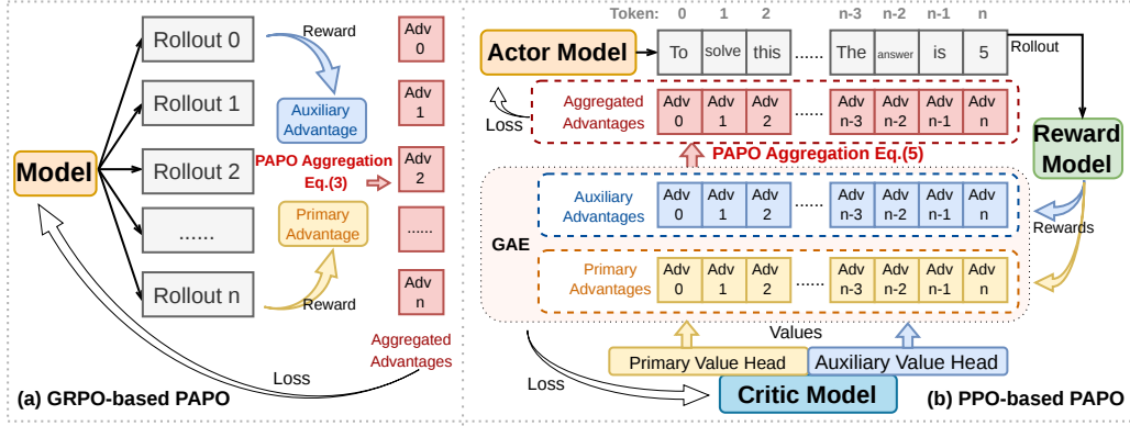
Figure 2: Overview. (a) GRPO-based PAPO. Given multiple rollouts, primary and auxiliary rewards are converted to sequence-level advantages and combined. (b) PPO-based PAPO. A multi-head critic estimates objective-specific values for the primary and auxiliary objectives. Token-level advantages are then computed using GAE and fused by PAPO before optimizing the actor.
