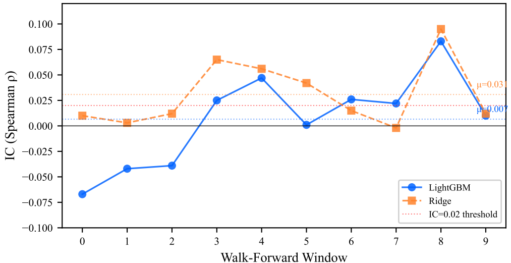
Figure 2: Per-Window IC Stability (US, 477 stocks)
