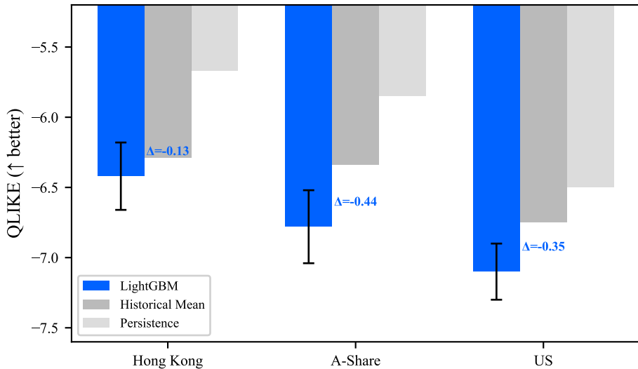
Figure 3: Cross-Market Volatility Prediction (QLIKE)
