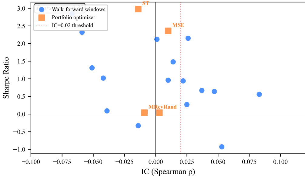
Figure 4: The Sharpe Paradox — IC vs Sharpe Decoupling
