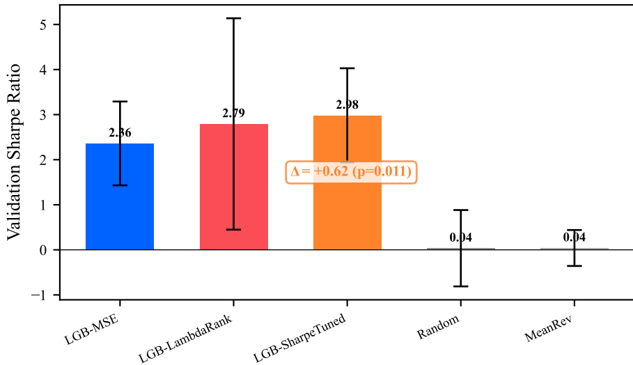
Figure 6: Portfolio Optimization — Method Comparison
