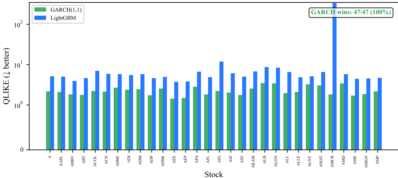
Figure 7: GARCH(1,1) vs LightGBM — Per-Stock QLIKE
