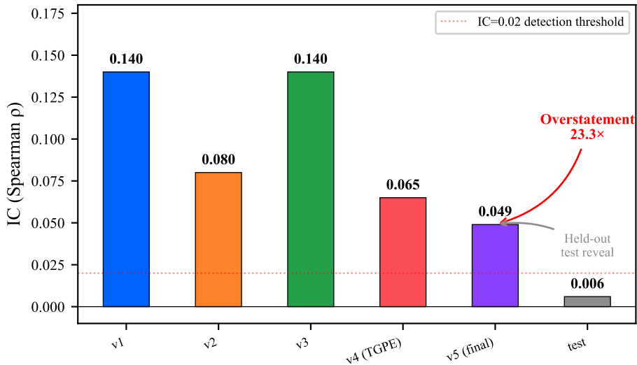
Figure 8: CTM IC Evolution — Bug Fixes Reveal Overfitting
