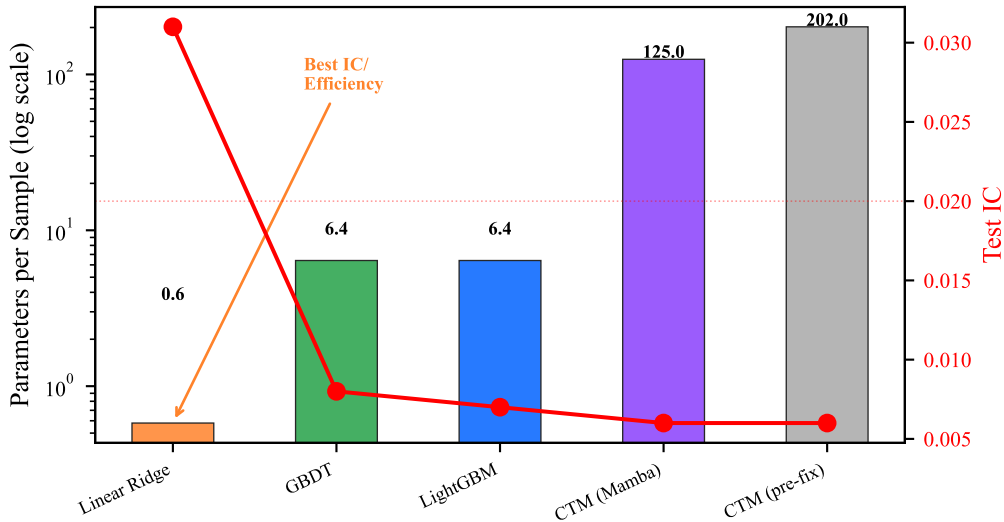
Figure B1: Parameter Efficiency vs Predictive Power
