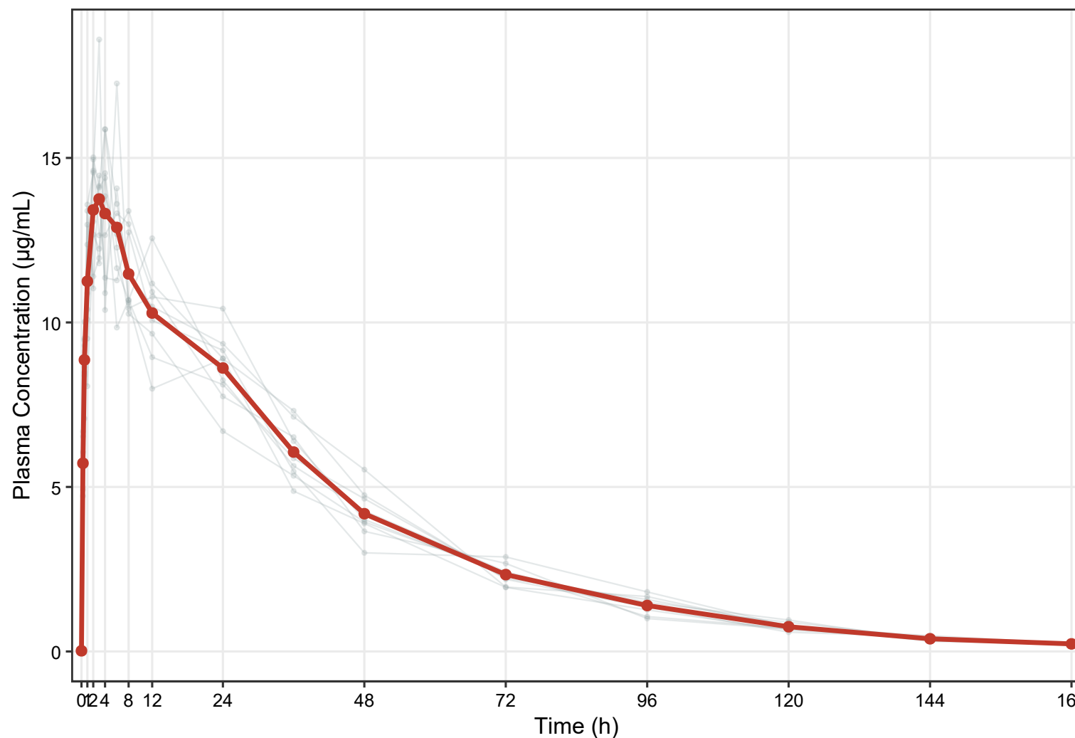
Individual Replicate Profiles with Mean Overlay
