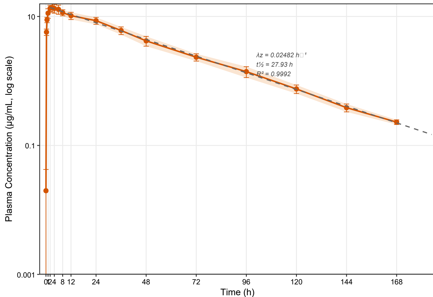
Terminal Phase Elimination Fit
