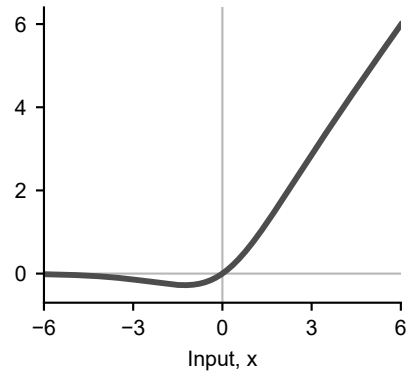
f SiLU / Swish
