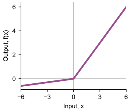
d Leaky ReLU ( \alpha = 0.1 )
