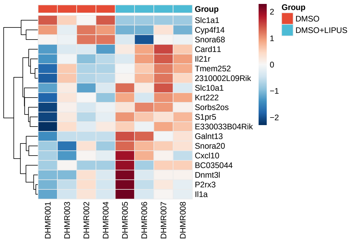
DEG heatmap (19 genes) |\log_2FC| \geq 1 , p \leq 0.05 , rowSum > 10
