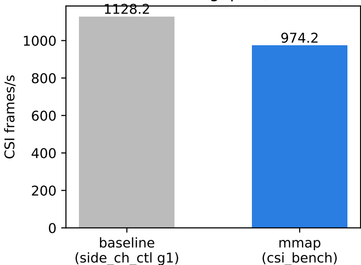
CSI frame throughput (frames/s)
