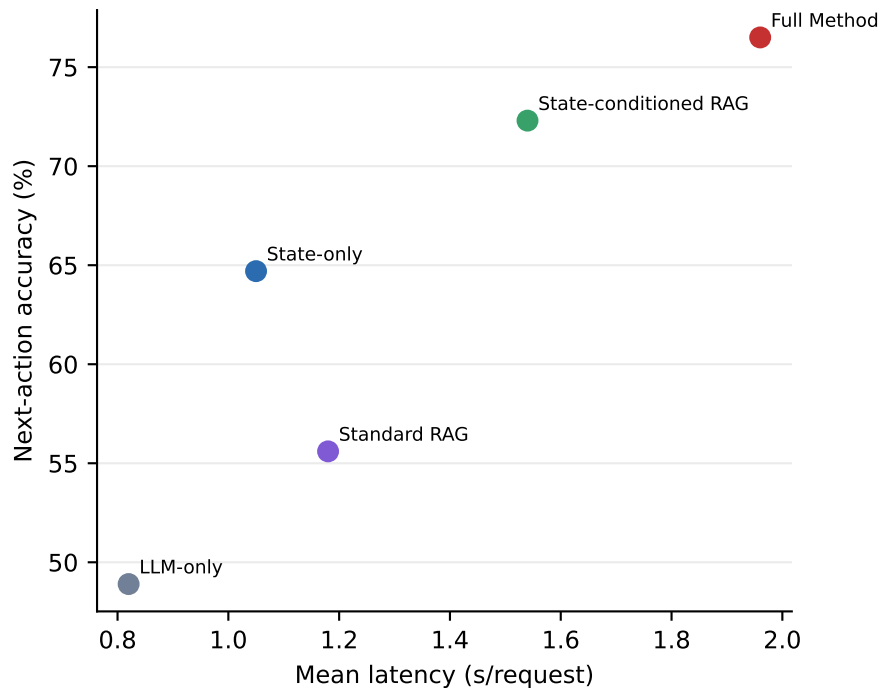
(a) EAI-VirtualHome
