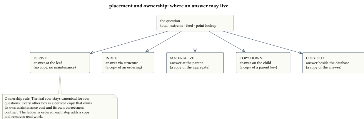
Figure 6: Placement and ownership: where an answer may live.
