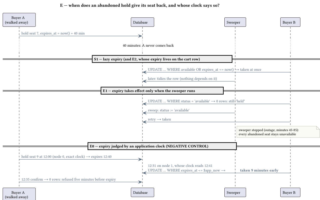
Figure 11: When an abandoned hold gives its seat back, and whose clock says so.
