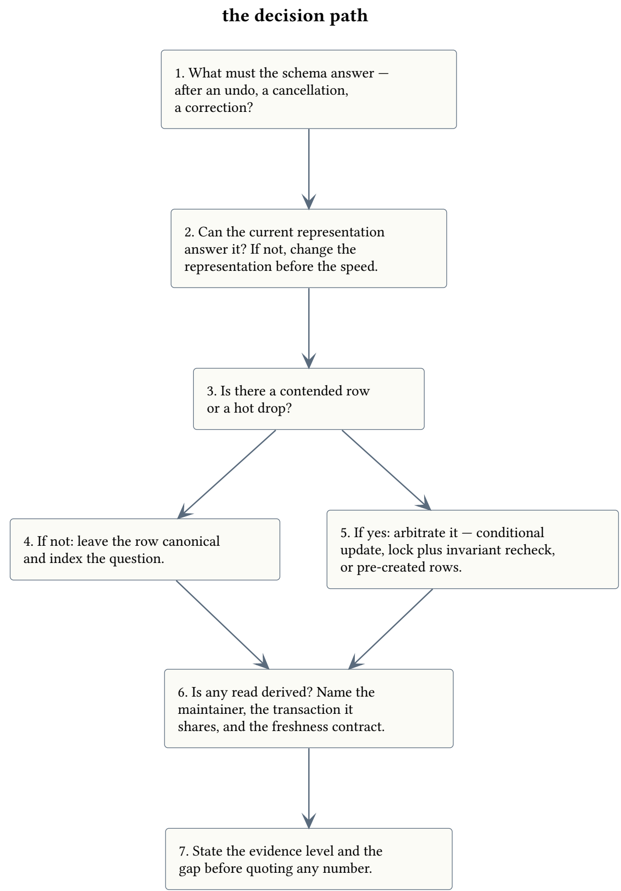
Figure 1: The decision path, in the order the decisions bind.
