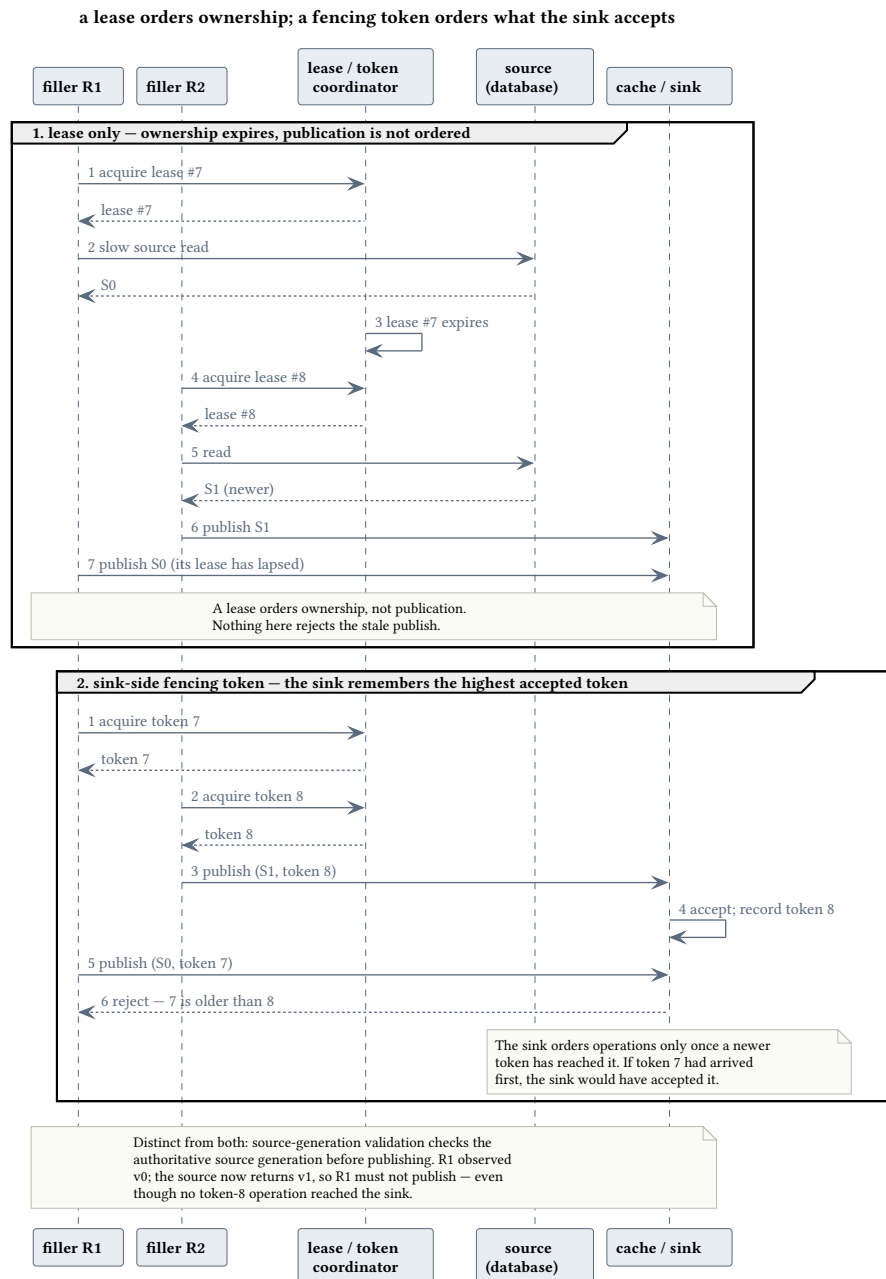
Figure 14: A lease orders ownership; a sink-side token and a source-generation check refuse the stale publish.
