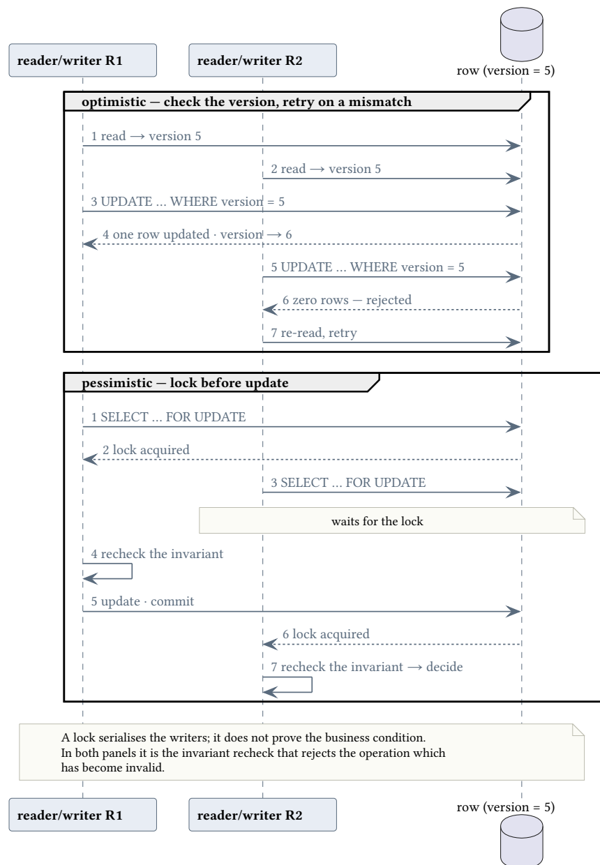
Figure 8: The invariant recheck, not the lock, rejects an operation that has become invalid.
