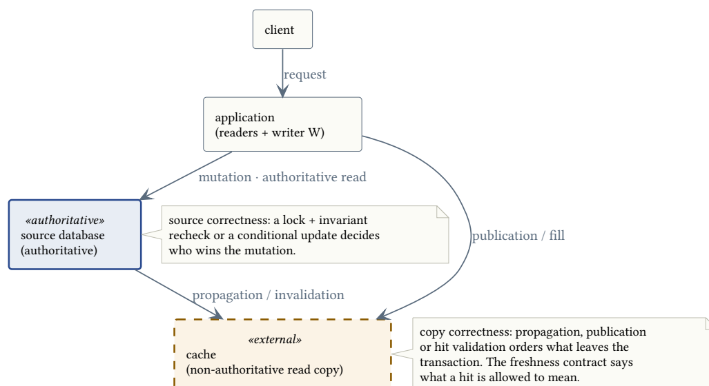
Figure 12: The cache is a non-authoritative read copy beside the authoritative database.
