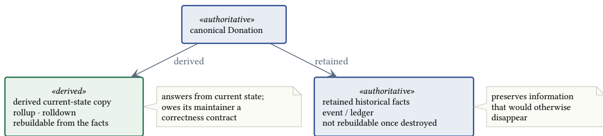
Figure 9: One canonical fact feeds a derived current-state copy or a retained history.
