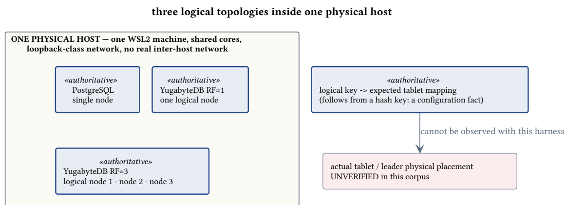
Figure 16: Logical multi-node topology; no real inter-host network was measured.
