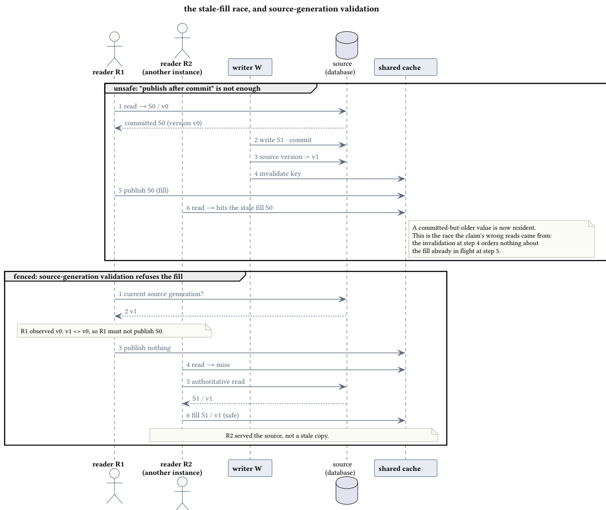
Figure 15: The stale-fill race, and the source-generation check that closes it.
