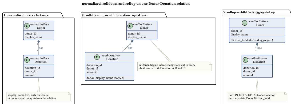
Figure 2: Normalized, rolldown and rollup on one parent-and-child relation.
