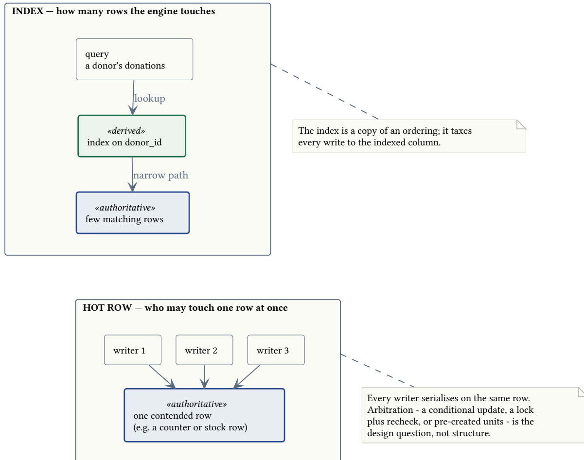
Figure 7: An index narrows the scan; a hot row serialises the writers.
