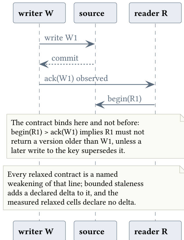
Figure 13: The strict-after-acknowledgement contract, and the point on the timeline where it binds.
