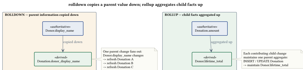
Figure 3: Rolldown fans a parent change out; rollup aggregates a child change up.
