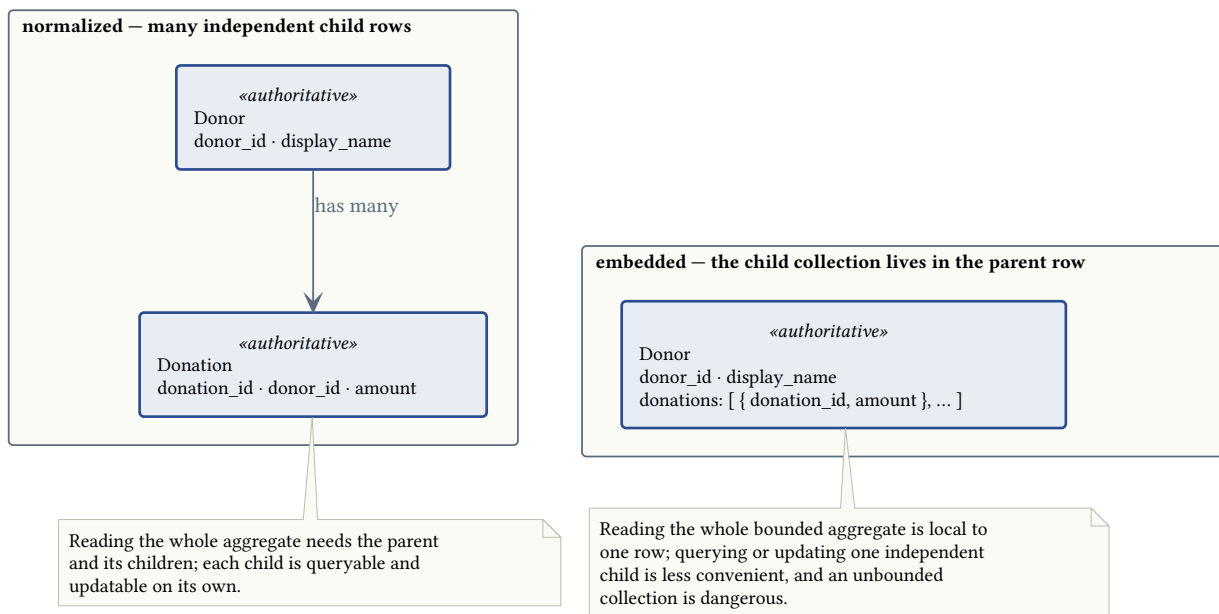
Figure 4: Normalized child rows beside a bounded child collection inside the parent.
