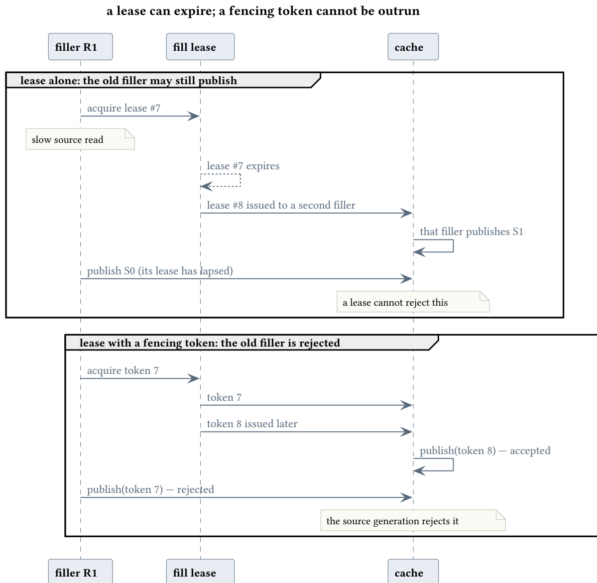
Figure 6: A lease can expire under a slow filler; a fencing token rejects the stale owner.
