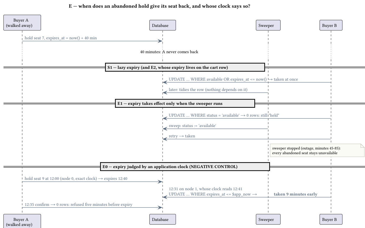
Figure 4: When an abandoned hold gives its seat back, and whose clock says so.
