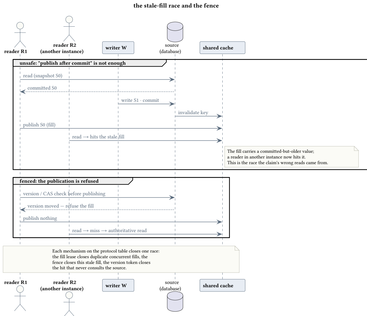
Figure 7: The stale-fill race, and the fence that closes it.
