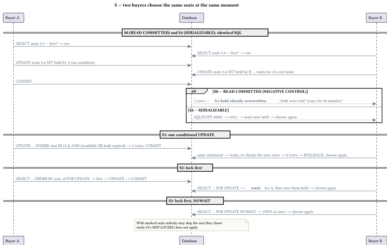
Figure 2: Two buyers choose the same marked seats at the same moment.
