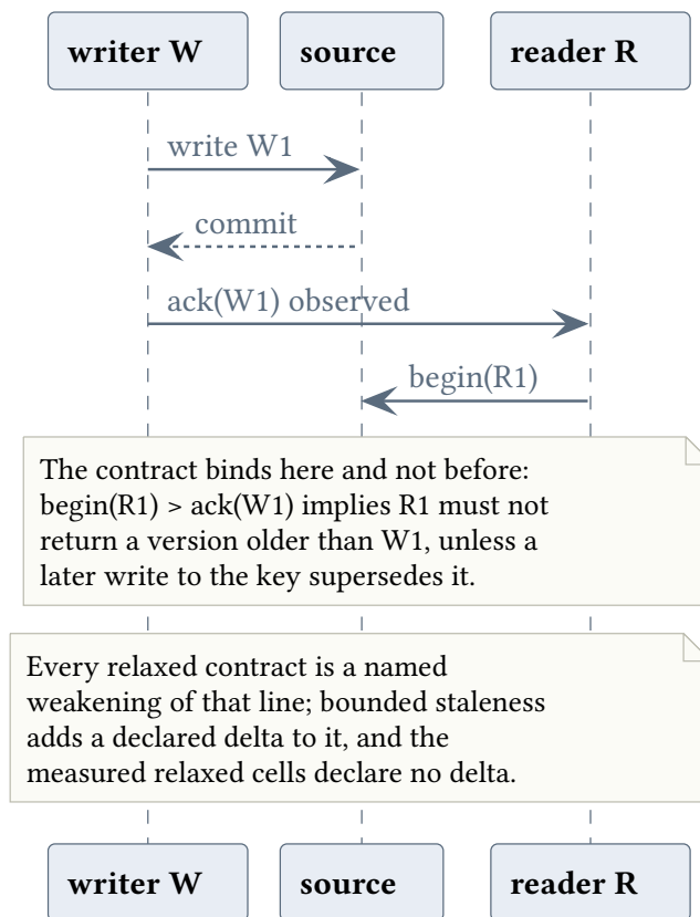
Figure 5: The strict-after-acknowledgement contract, and the point on the timeline where it binds.
