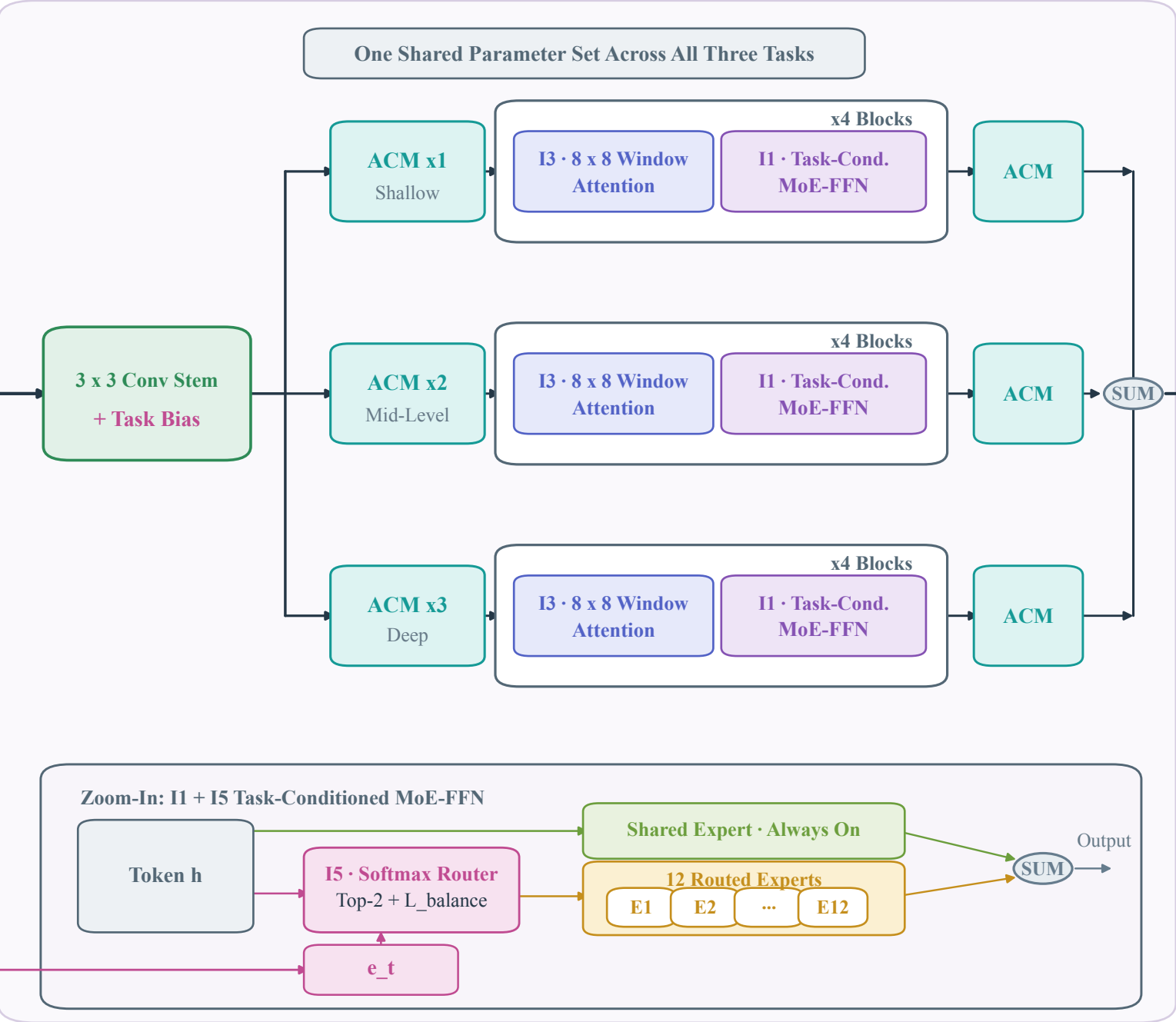
B Multi-Scale U-MoE Backbone
