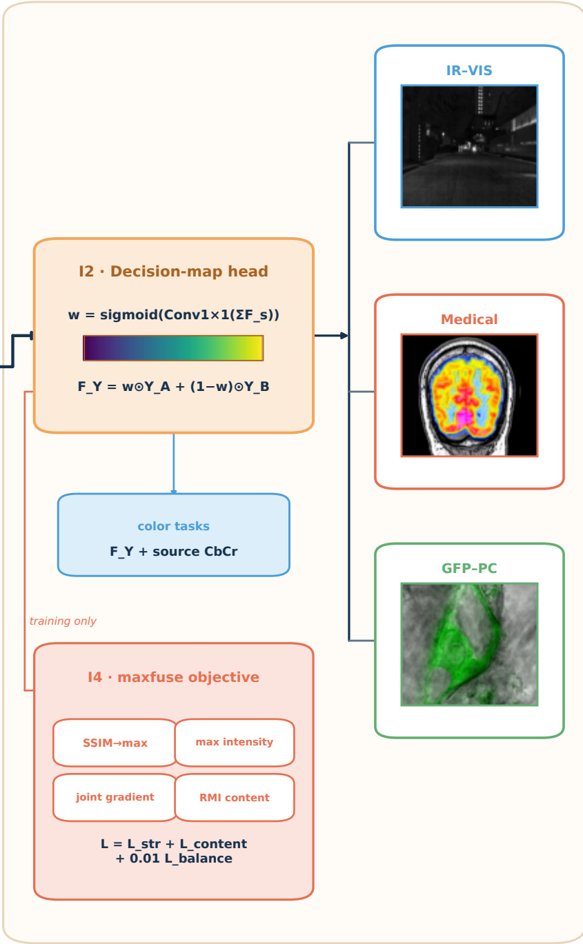
C Decision-map fusion and outputs
