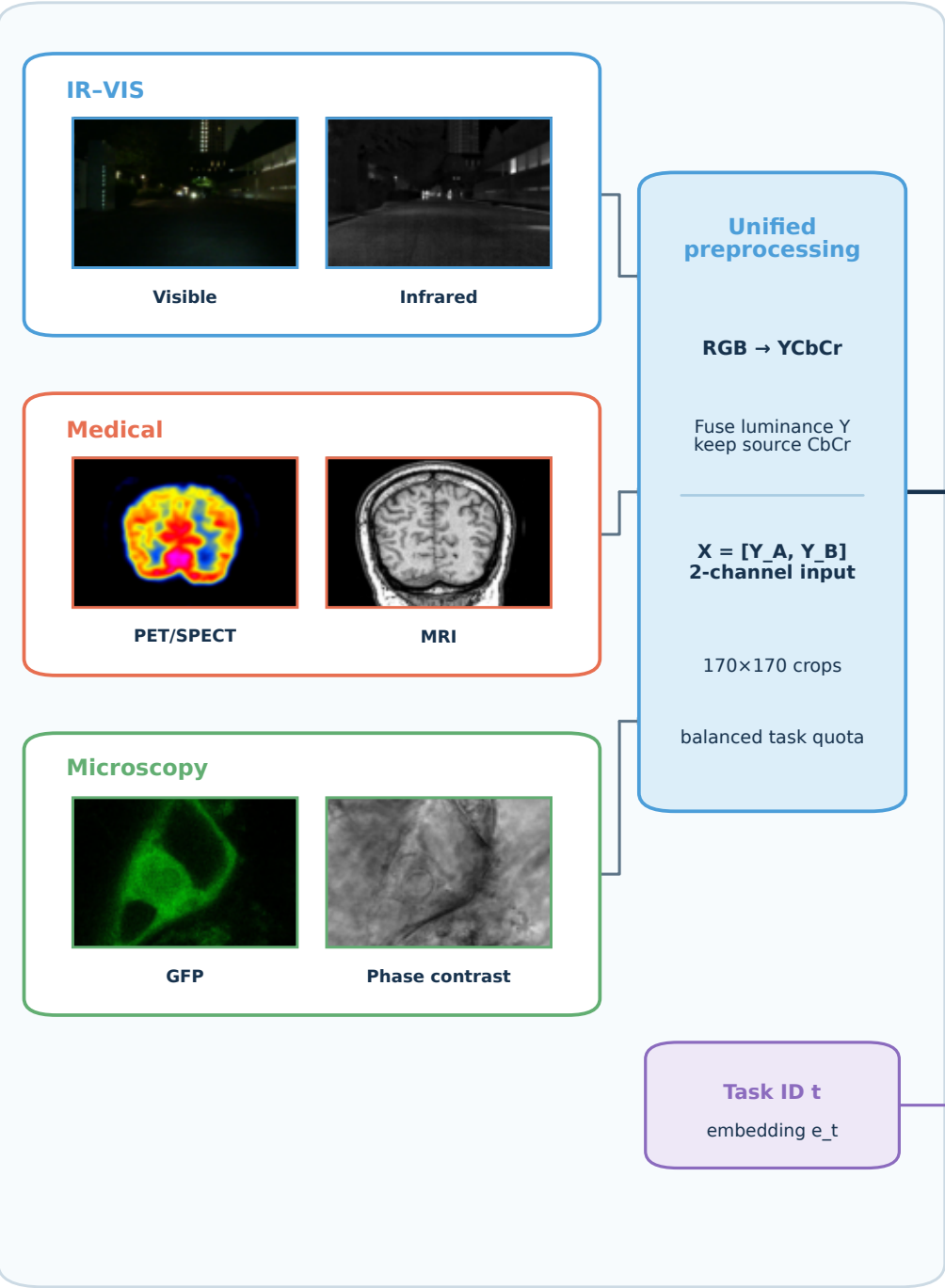
A Unified multi-task input
