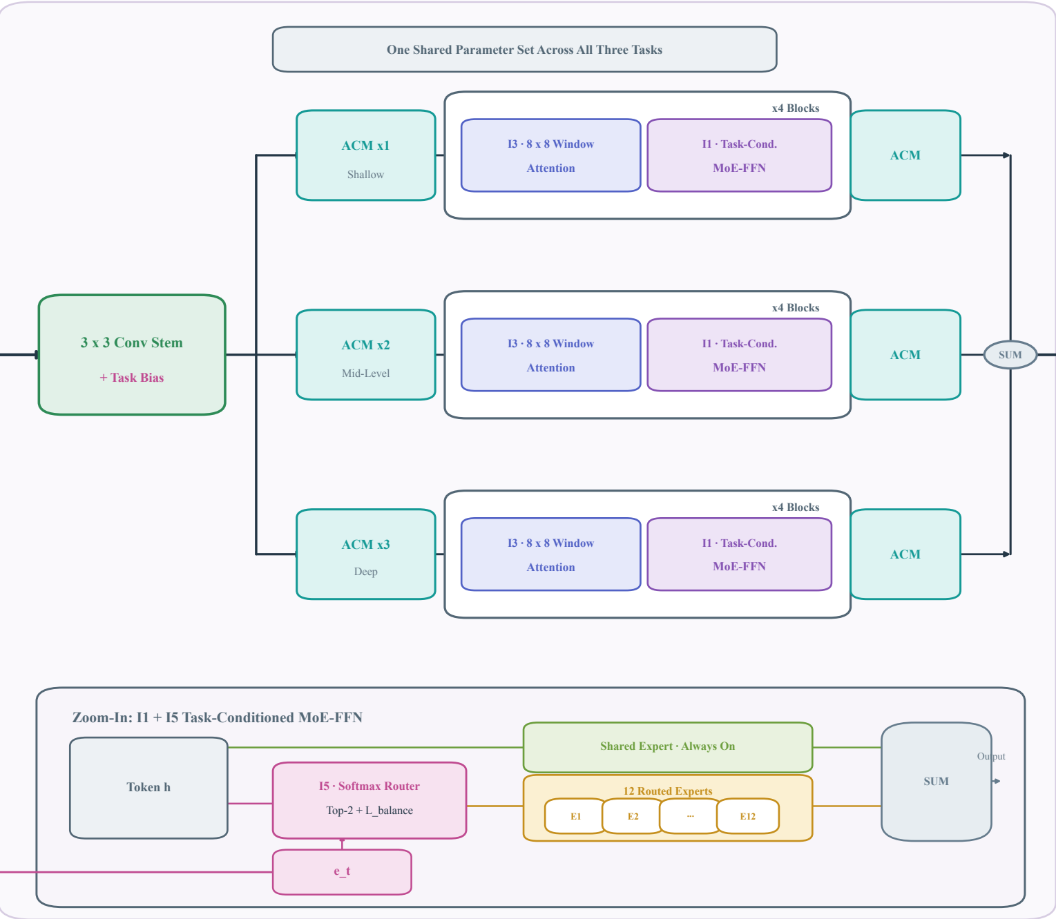
B Multi-Scale U-MoE Backbone
