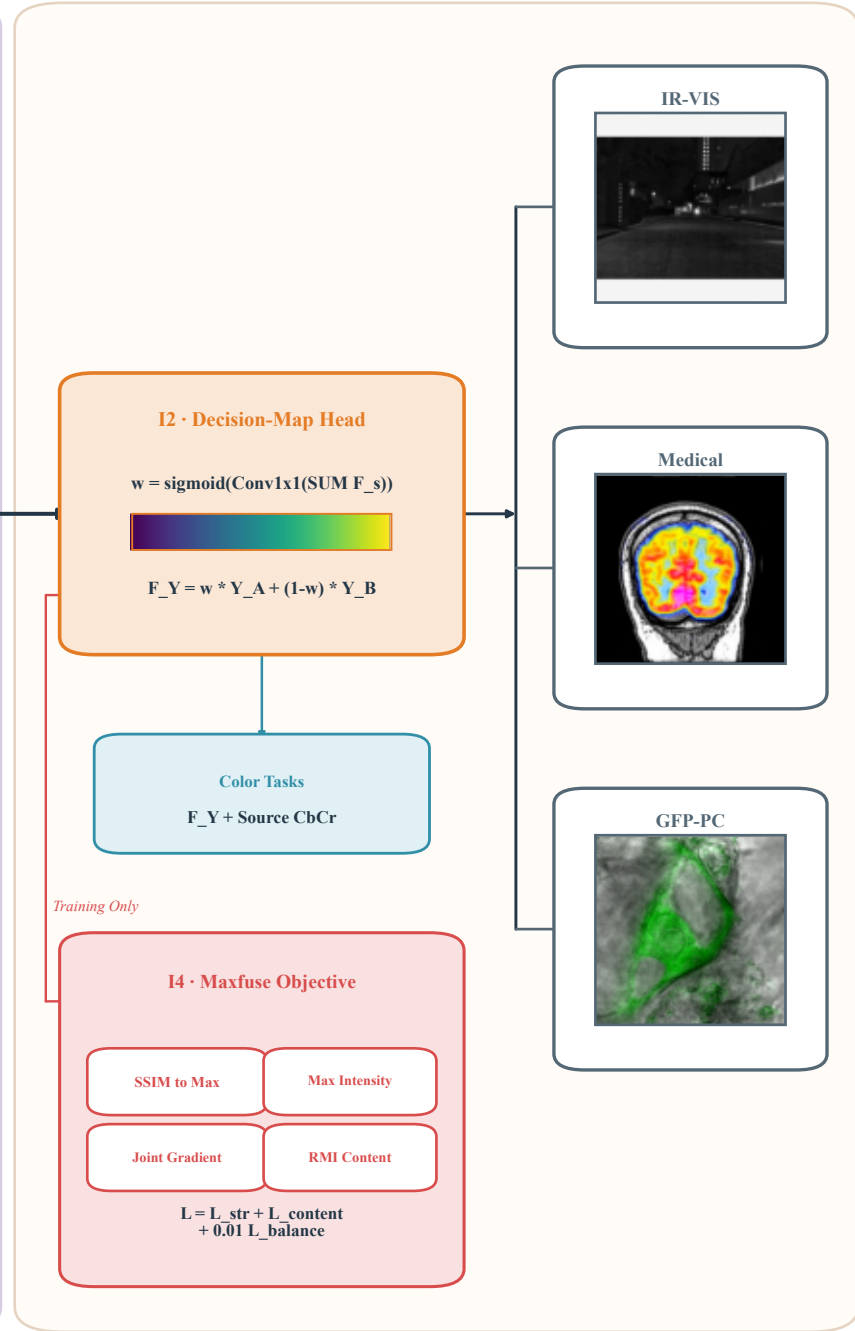
Efficient Training
