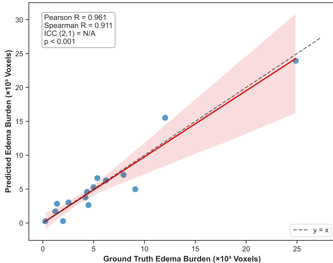
Correlation Analysis - best_model
