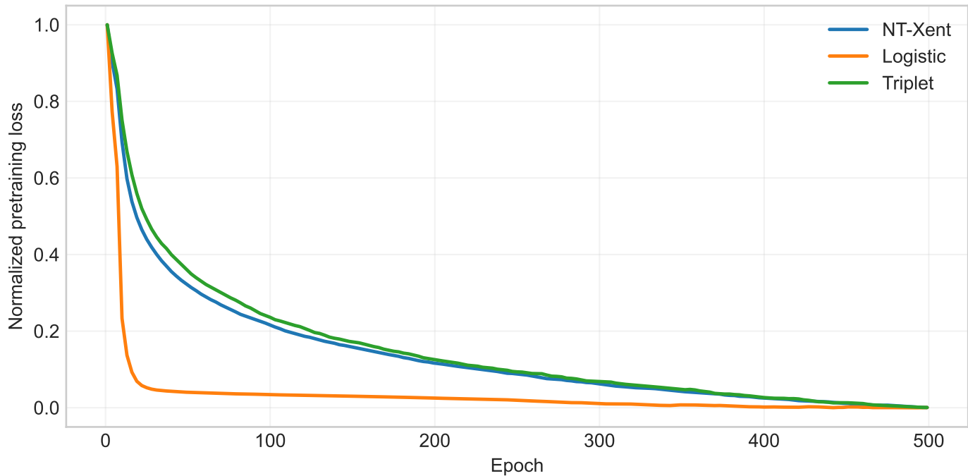
Contrastive-loss pretraining curves
