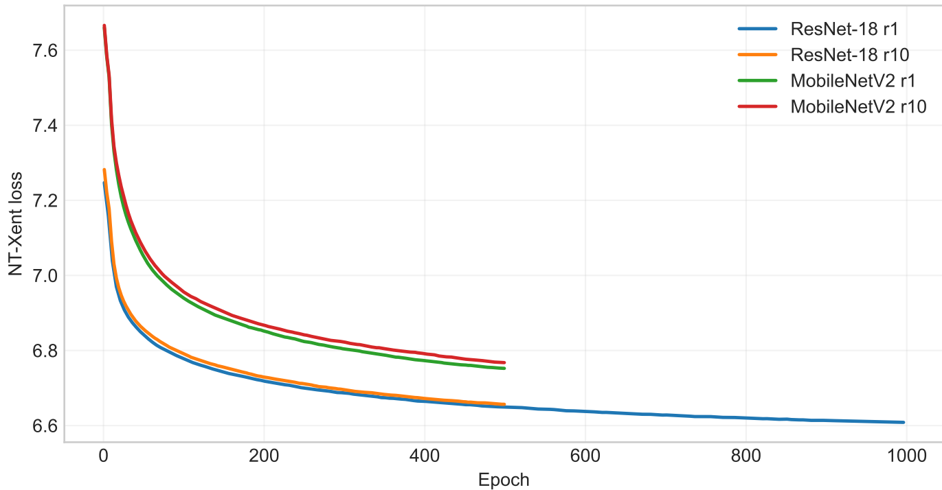
Main SimCLR pretraining curves
