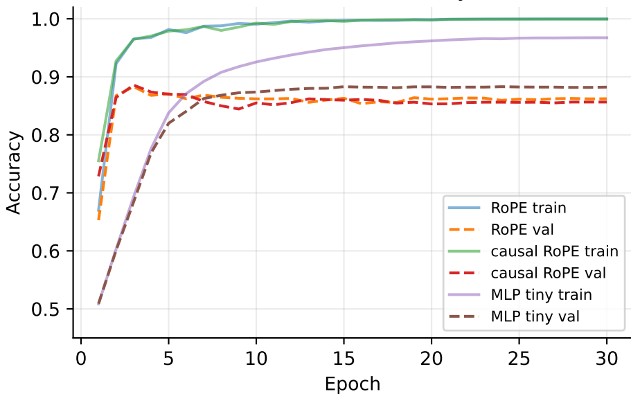
Causal/MLP Accuracy
