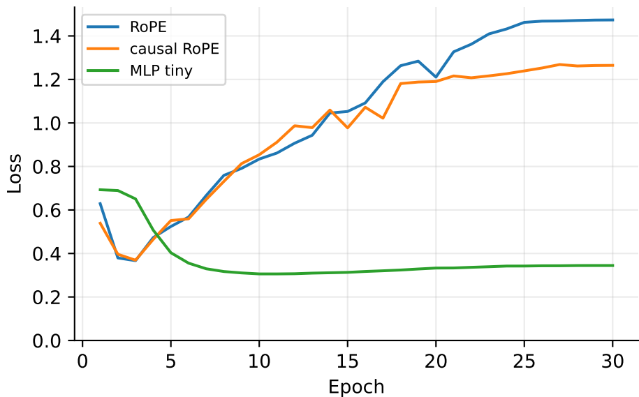
Causal/MLP Validation Loss
