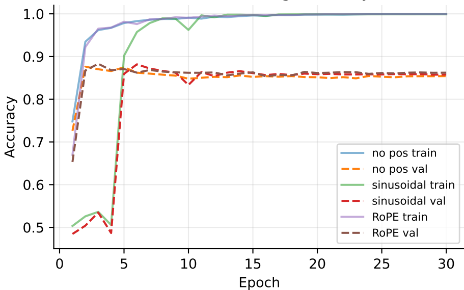
Position Encoding Accuracy
