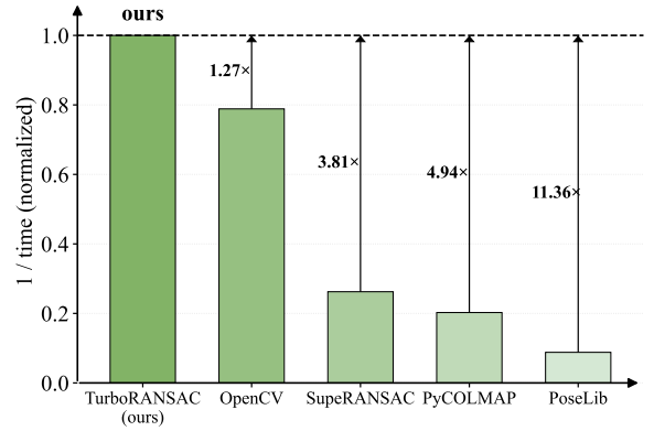
Fig. 1: Runtime comparison of different methods.
