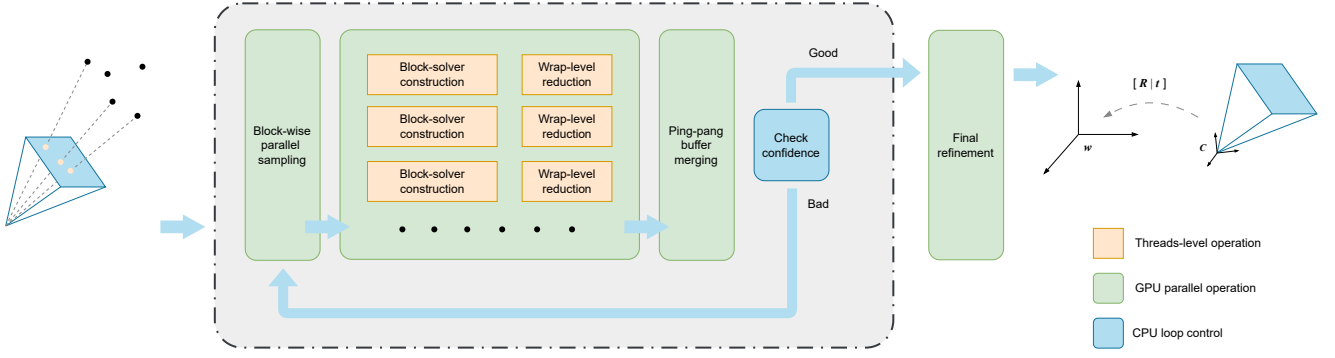
Fig. 2: The overall architecture of the proposed TurboRANSAC framework.
