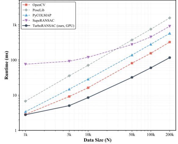
Fig. 4: Runtime for pose estimation on synthetic data.
