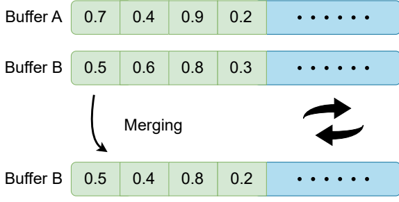
Fig. 3: Pairwise merge under ping-pong buffering.
