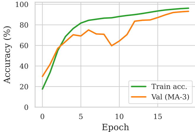
(b) Classification accuracy
