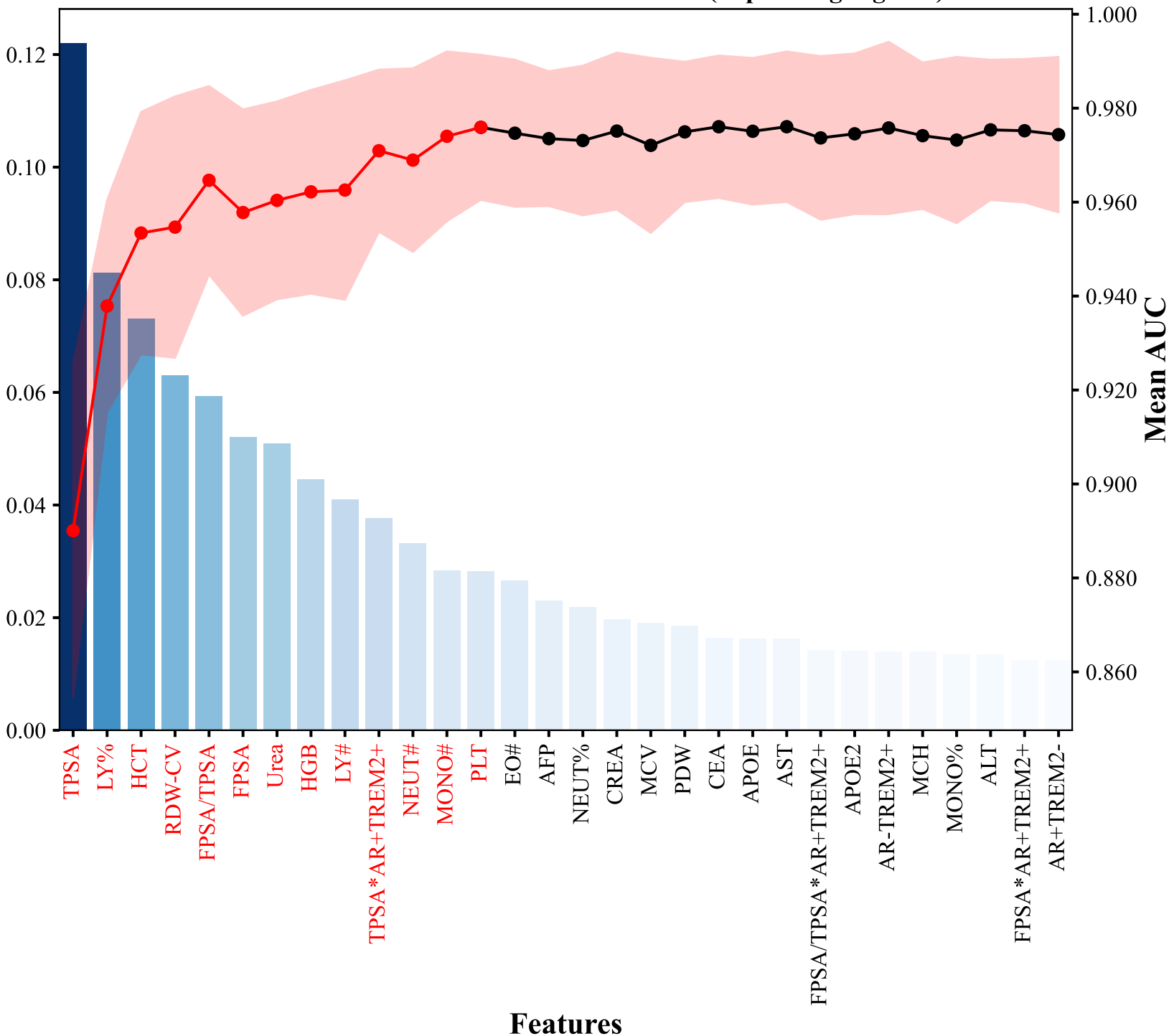
Feature Contribution and AUC Performance (Top 13 Highlighted)
