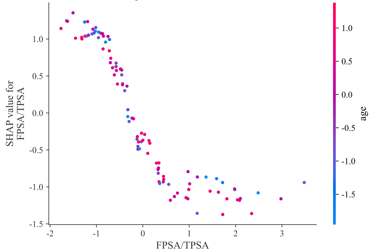
SHAP Dependence Plot for FPSA/TPSA
