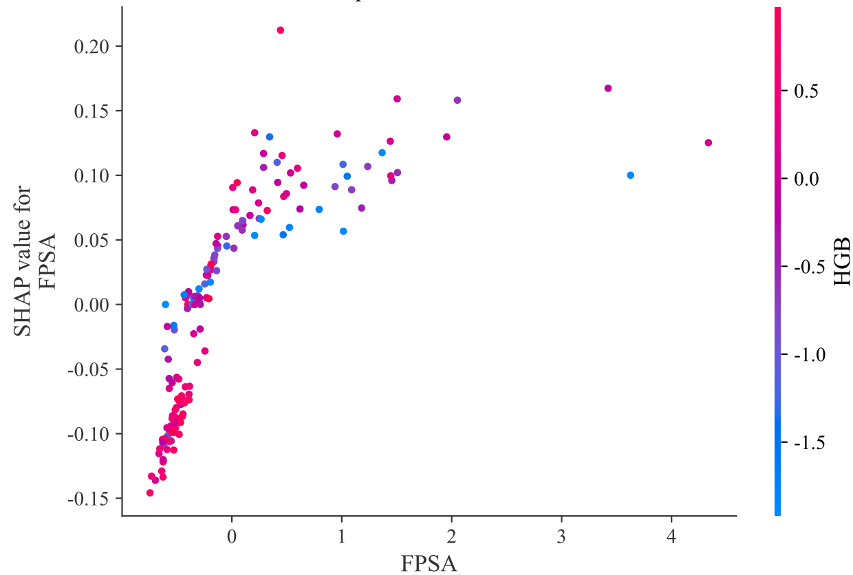
SHAP Dependence Plot for FPSA
