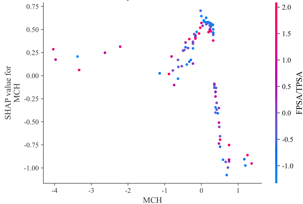
SHAP Dependence Plot for MCH
