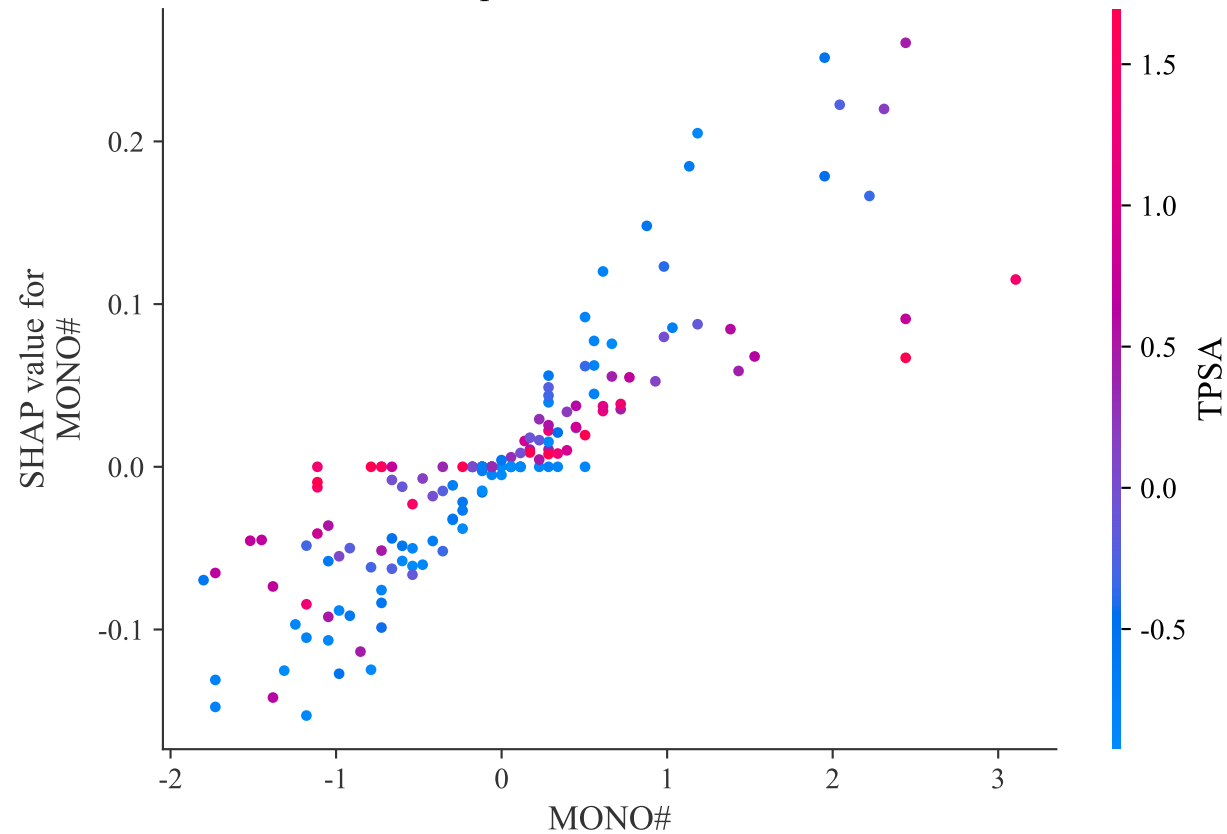
SHAP Dependence Plot for MONO#
