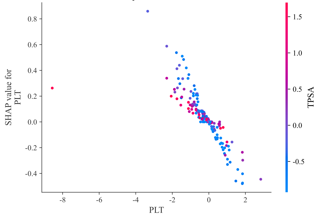
SHAP Dependence Plot for PLT
