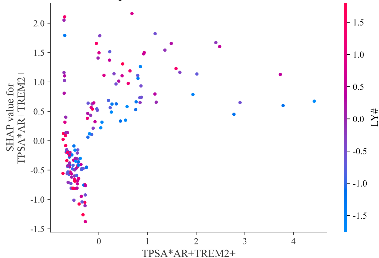
SHAP Dependence Plot for TPSA*AR+TREM2+
