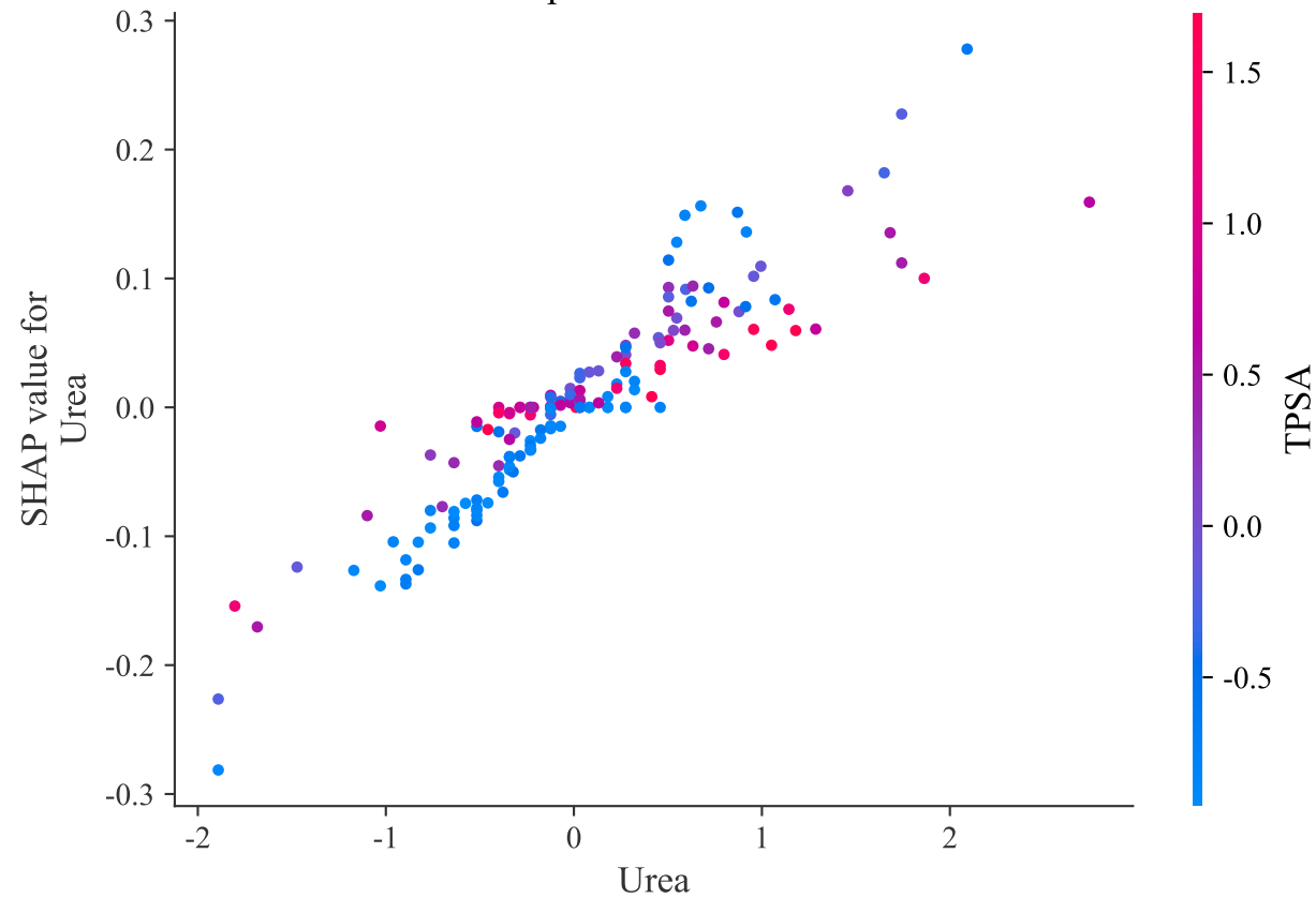
SHAP Dependence Plot for Urea
