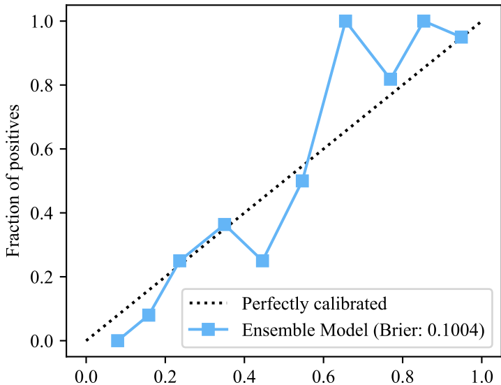
Calibration plots (Reliability curve)
