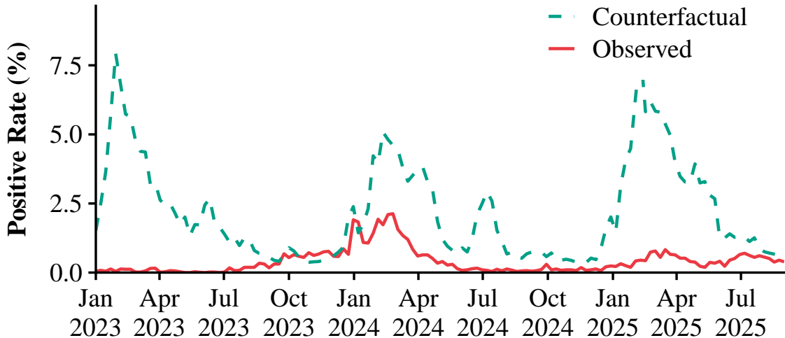
Observed vs Predicted (Influenza B)
