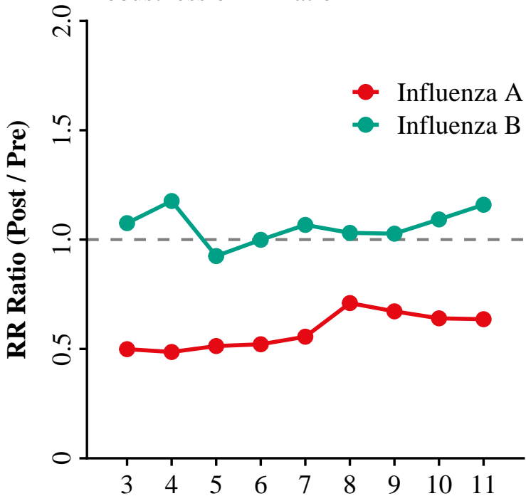
Robustness of RR ratio
