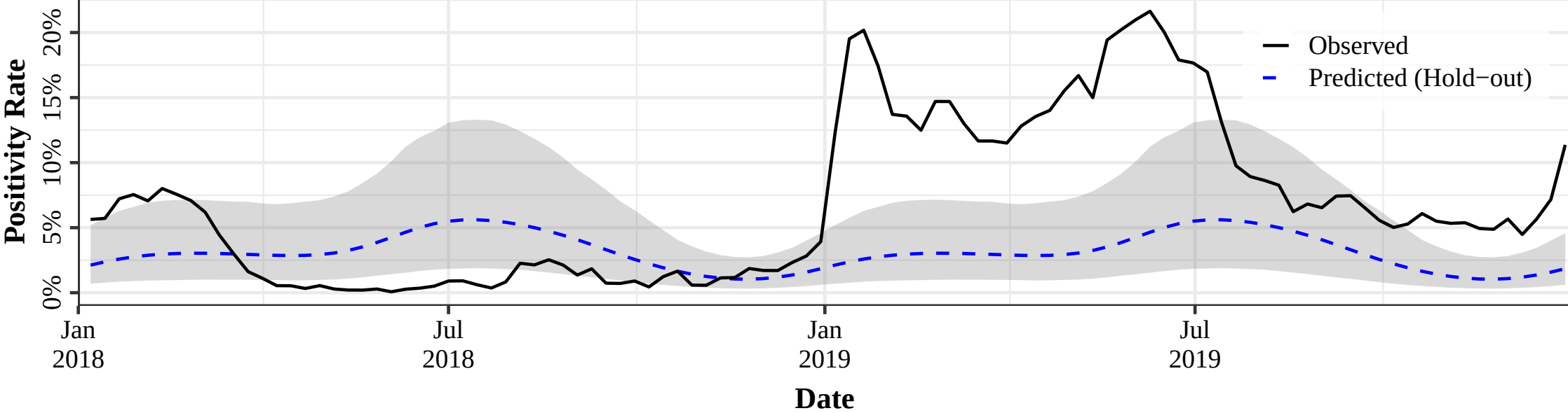
Sensitivity Analysis: Negative Control (Predicting 2018–2019)
