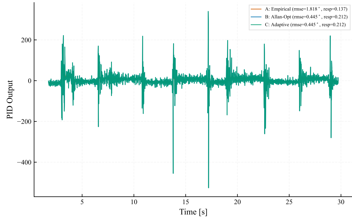
Roll: PID Control (setpoint=0 °)
