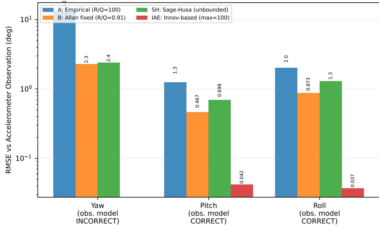
Three-Channel Cross-Validation: Kalman Filter RMSE Comparison
