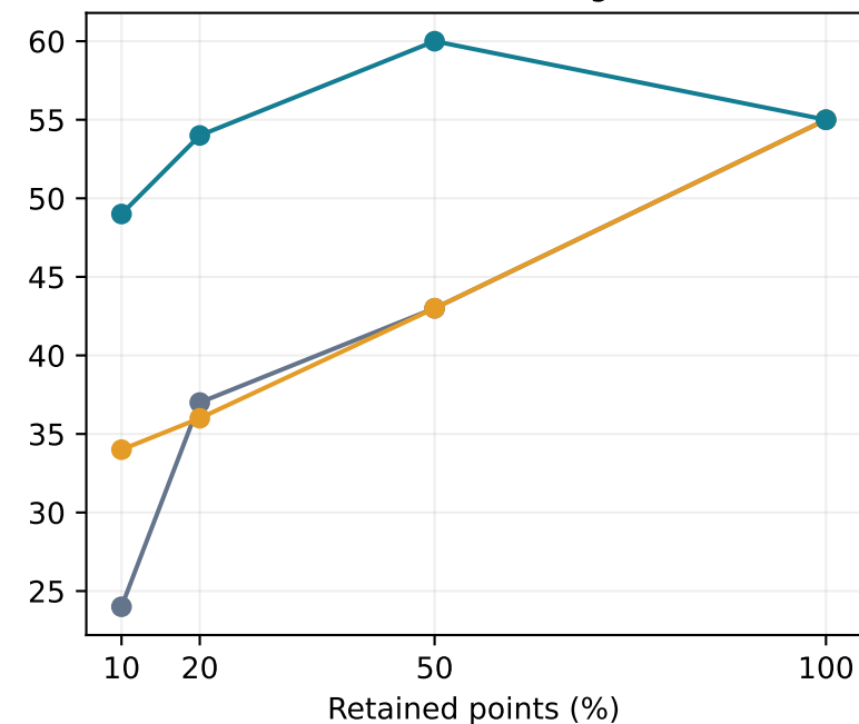
Spearman rho = 0.083
