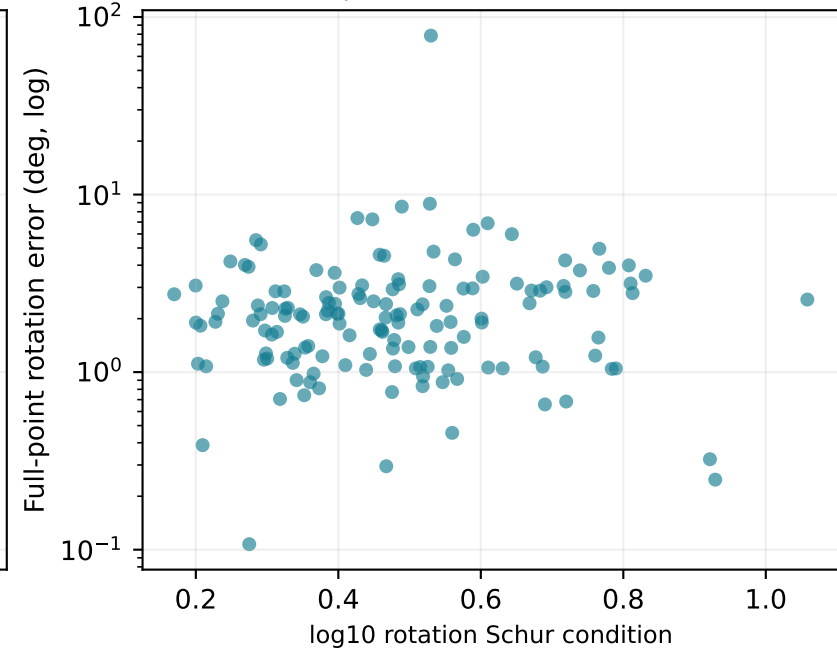
Spearman rho = 0.083
