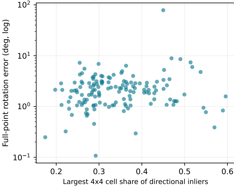
Spearman rho = 0.122
