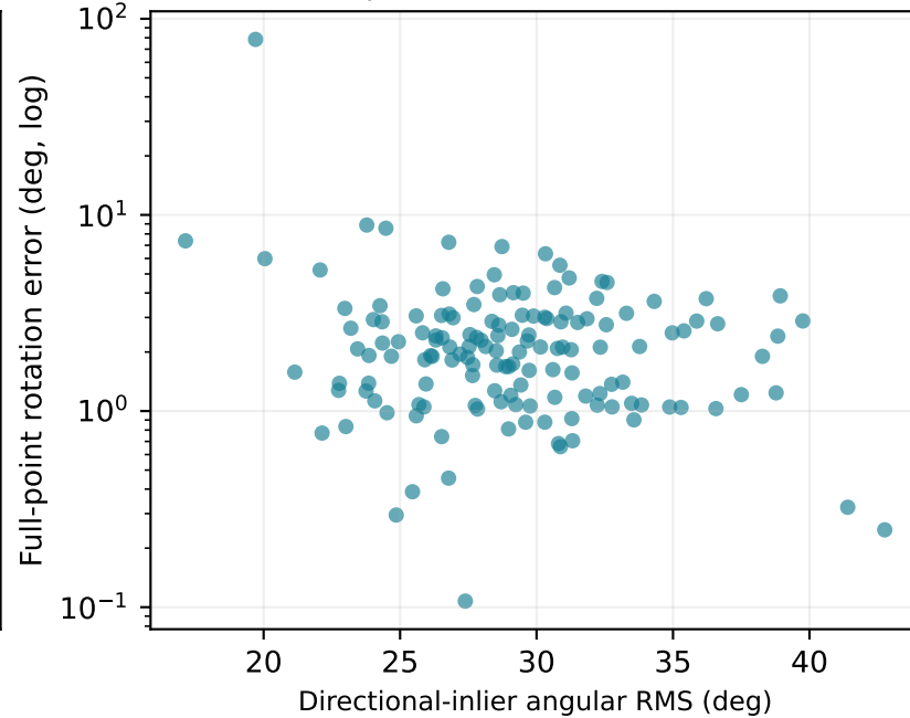
Spearman rho = -0.067
