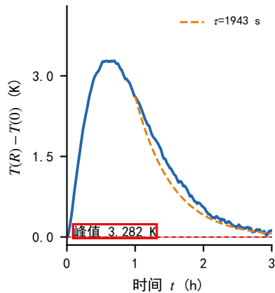
(c) 径向温差衰减
