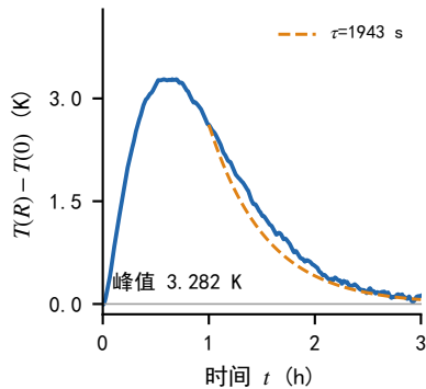
(c) 径向温差衰减
