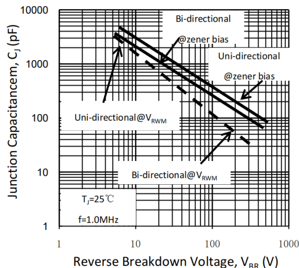
Fig. 6-Typical Junction Capacitance
