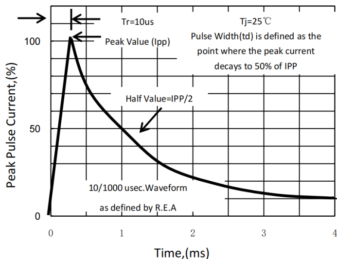
Fig. 5-Pulse Waveform
