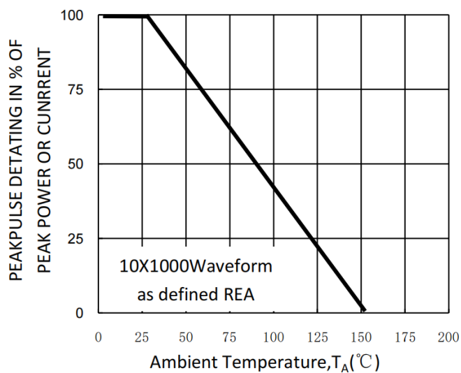
Fig. 1-Pulse Derating Curve
